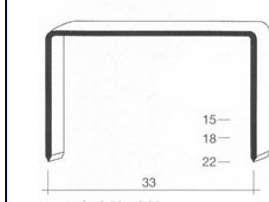
GRAPA 35 (BOXER)
