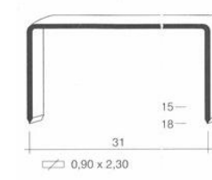
GRAPA 34 (2002-GRAP)
