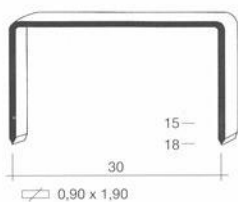
GRAPA 32 (CLINCHER)
